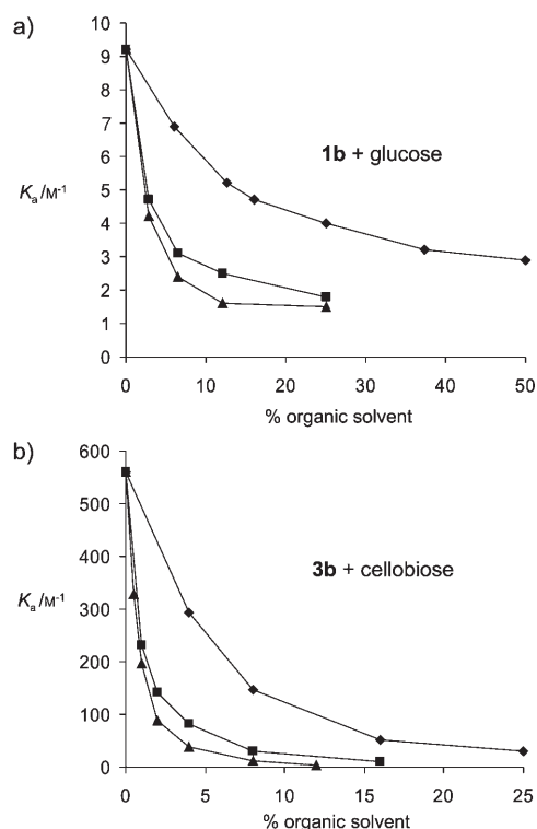
Figure 3. Binding constants ( K_a ) of synthetic receptors to carbohydrate substrates in water/organic solvent mixtures. Organic solvents: \blacklozenge = MeOH, \blacksquare = DMSO, \blacktriangle = MeCN. a) Association constants for 1b +glucose measured by ^1H NMR spectroscopy (deuterated solvents). b) Association constants for 3b +cellobiose measured by fluorescence spectroscopy (data for MeOH is repeated from Figure 2a).
